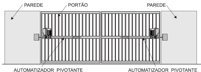
VISTA FRONTAL
