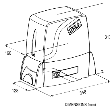
DIMENSIONS (mm)
